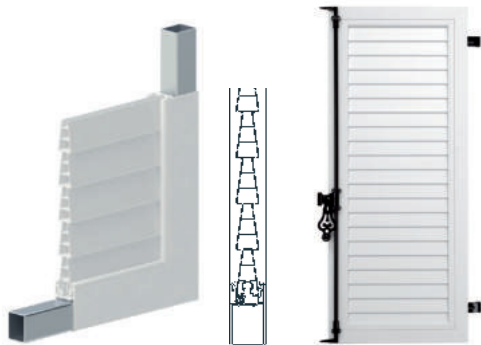
Lames jointives alizé
